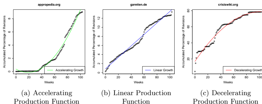
Fig. 2. Types of Production Functions: The x -axes in all three plots depict the time in weeks up to two years, while the y -axes depict the accumulated amount of activity during each corresponding week. The lines in each plot represent the best fitted linear or quadratic function for the observed data (circles).
